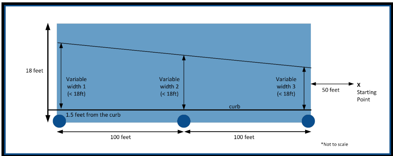
Figure C.0.1 Schematic of Survey Site
